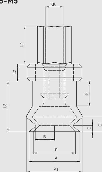
PZVC-10-KN-M5 PZVC-10-KS-M5
