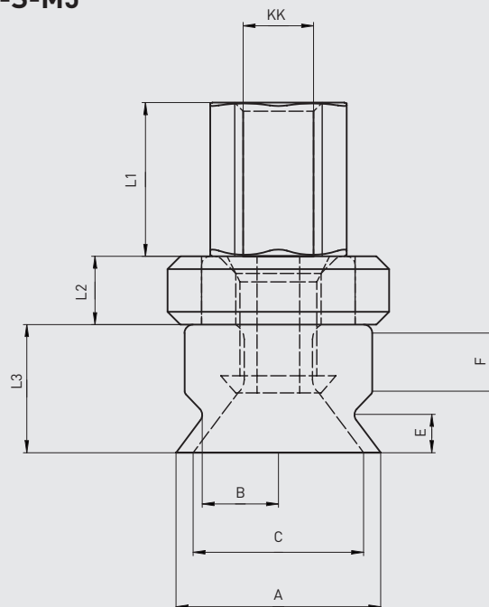
PZVC-10-KN-M5 PZVC-10-KS-M5
